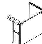
End Bench to Full Modesty or Half Modesty with Full End Panel or Open Leg End Panel
